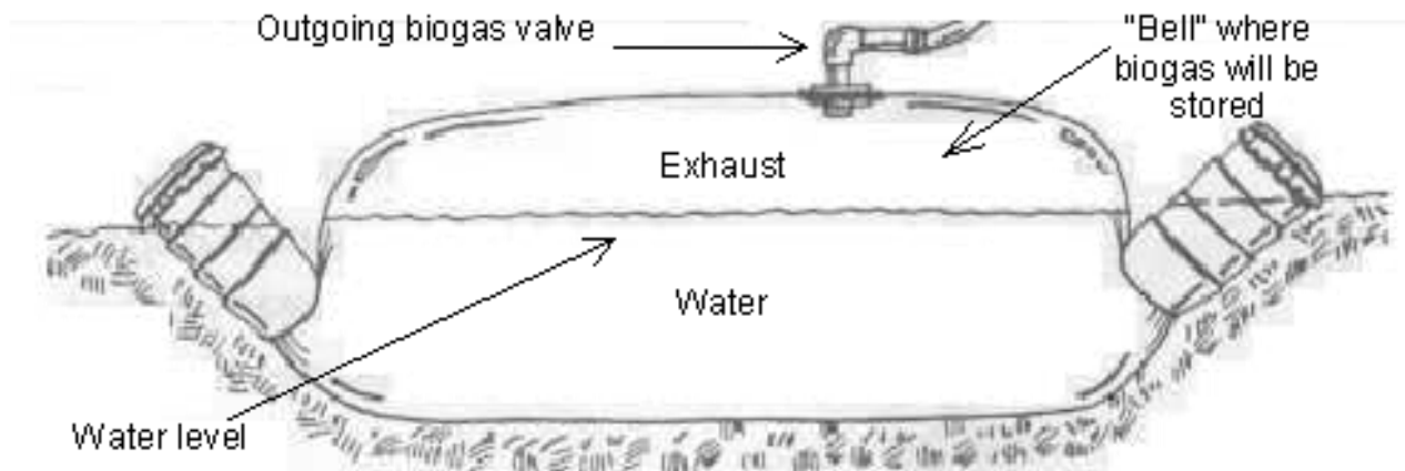
Figure 11. Diagram of a biogas plant, full of exhaust and water. Water represents 75% of the total volume of the bag. The other 25% is full of exhaust.
