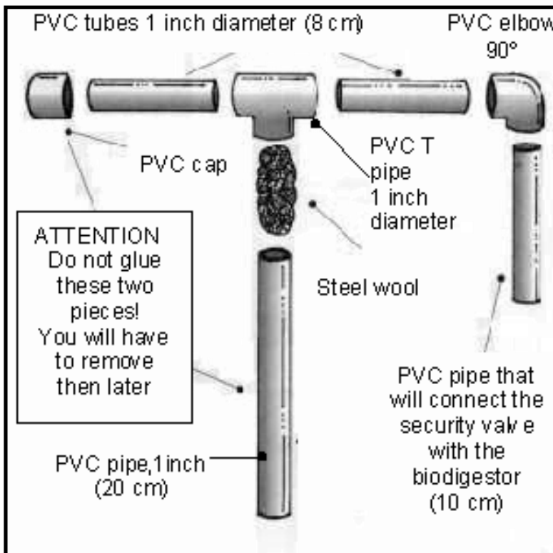
Figure 7. Diagram of the security valve.
