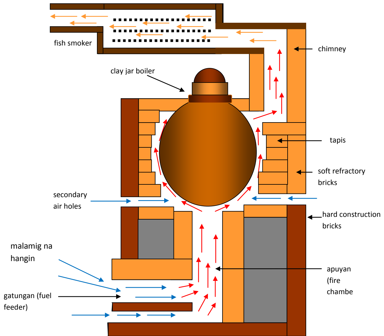
Cross section diagram of the Intermediate Wine Distillery. Joshua B. Guinto, Tagsibol Development Enterprises. September 2012
