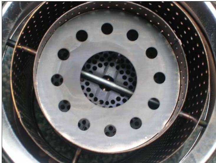
Fig. 2: Bottom view of the inner chimney nested in the outer chimney. The inner chimney has baffles at the bottom.
